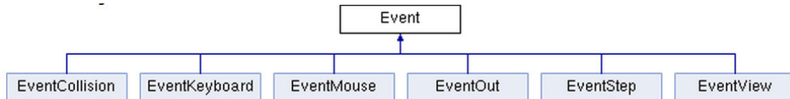
Figure 4.2: Dragonfly events
